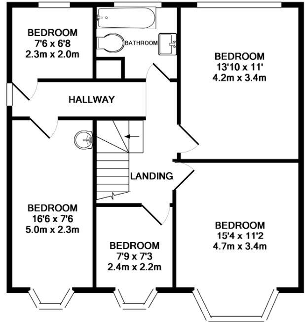
1ST FLOOR
