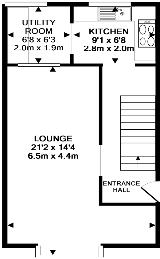
GROUND FLOOR APPROX. FLOOR AREA 388 SQ.FT. (36.1 SQ.M.)
