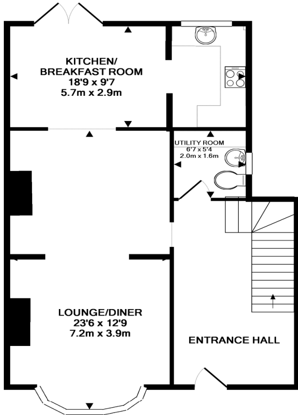
GROUND FLOOR APPROX. FLOOR AREA 699 SQ.FT. (64.9 SQ.M.)
