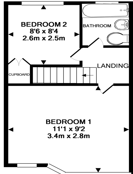
1ST FLOOR
