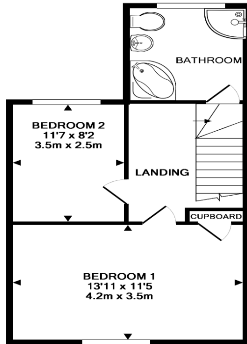
1ST FLOOR APPROX. FLOOR AREA 458 SQ.FT. (42.5 SQ.M.)
