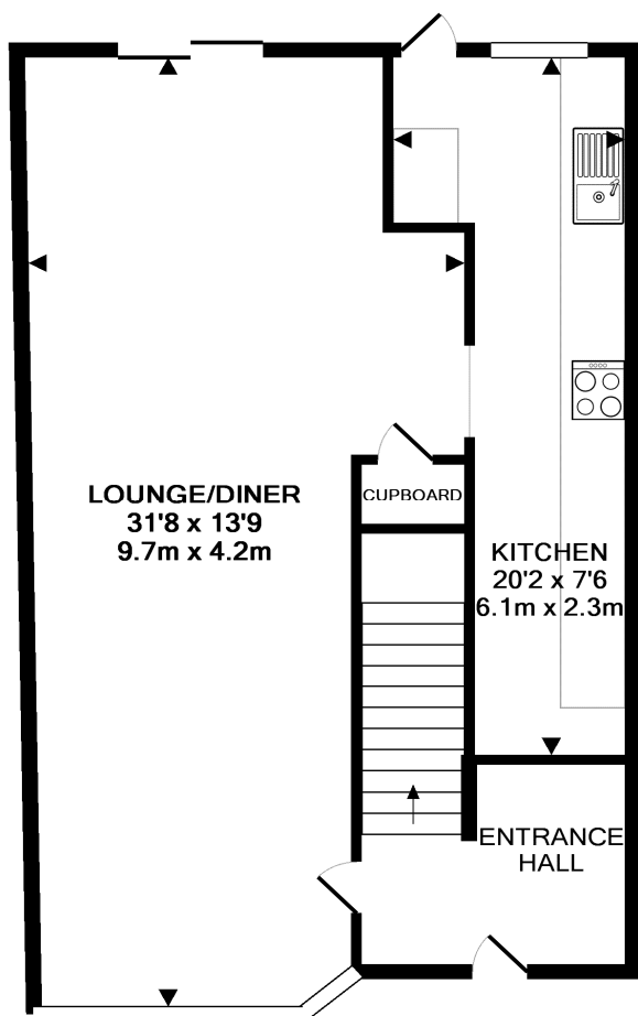
GROUND FLOOR APPROX. FLOOR AREA 576 SQ.FT. (53.5 SQ.M.)
