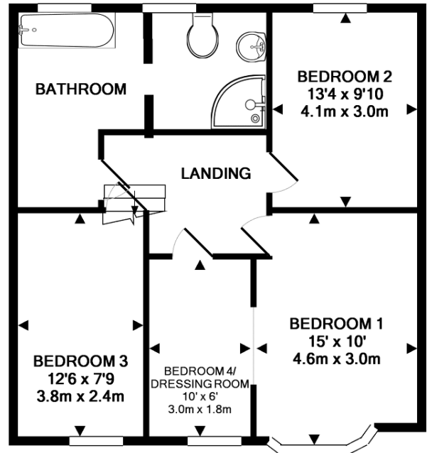
1ST FLOOR APPROX. FLOOR AREA 513 SQ.FT. (47.7 SQ.M.)
