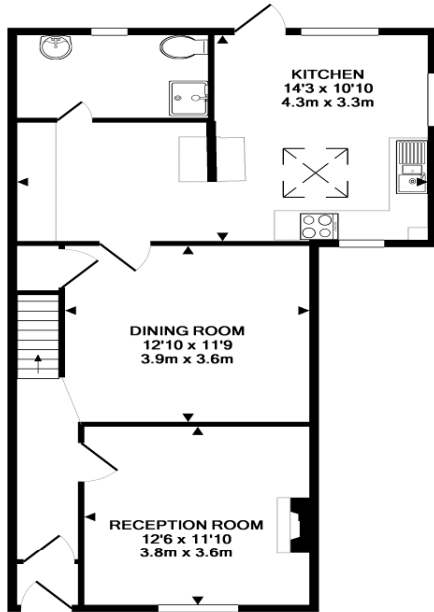
GROUND FLOOR APPROX. FLOOR AREA 685 SQ.FT. (63.6 SQ.M.)
